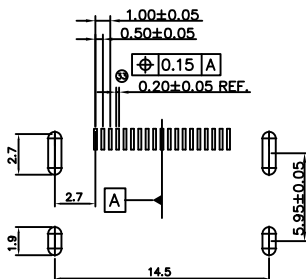
RECOMMENDED PCB LAYOUT TOL: ±0.05
