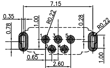
RECOMMENDED P.C.B. LAYOUT TOP VIEW (TOLRANCE: ±0.05)
