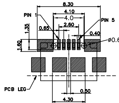
RECOMMENDED P.C.B. LAYOUT TOP VIEW (TOLERANCE: ±0.05)
